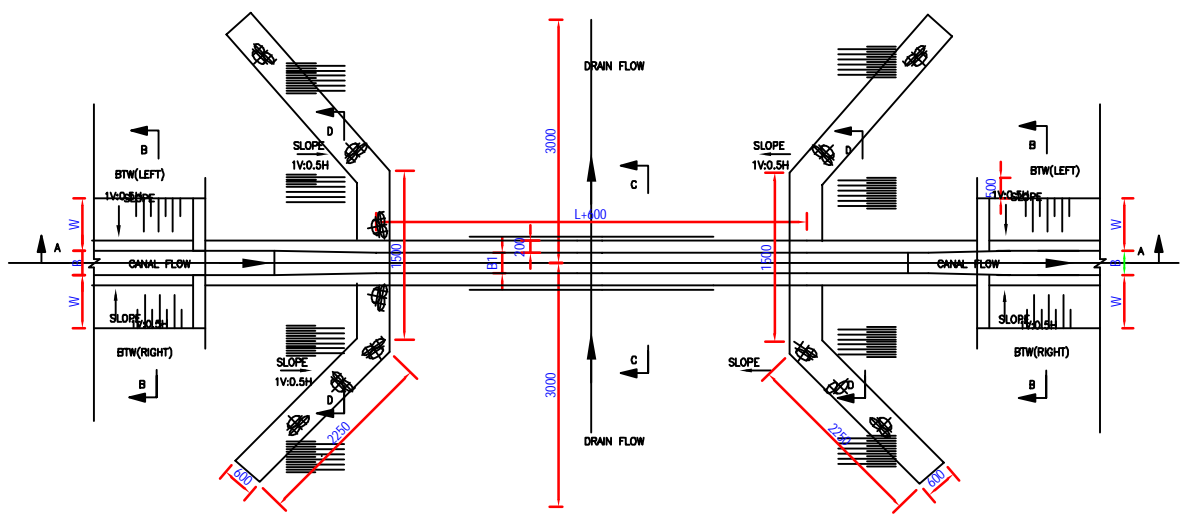
PLAN OF AQUEDUCT
