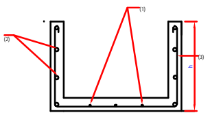
Span 3m to 5m
