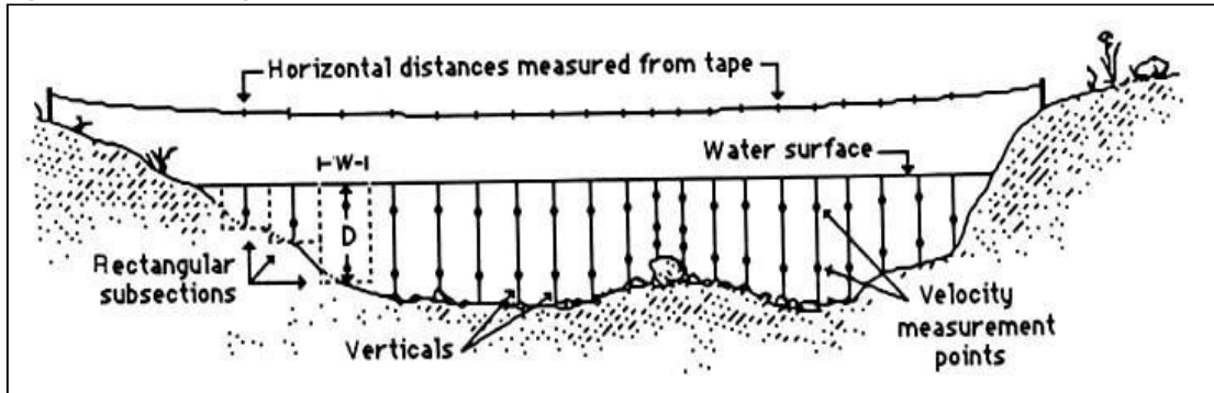
Figure 3-2: Discharge Measurement with Float Method
