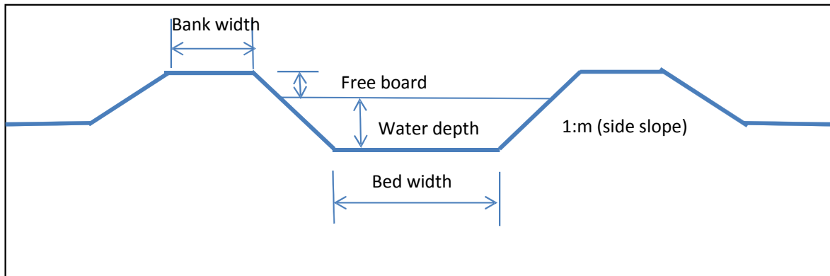
Figure 5-1: Typical Canal Section
