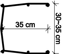
8 SWG Gabion Wire @ 20 cm c/c
